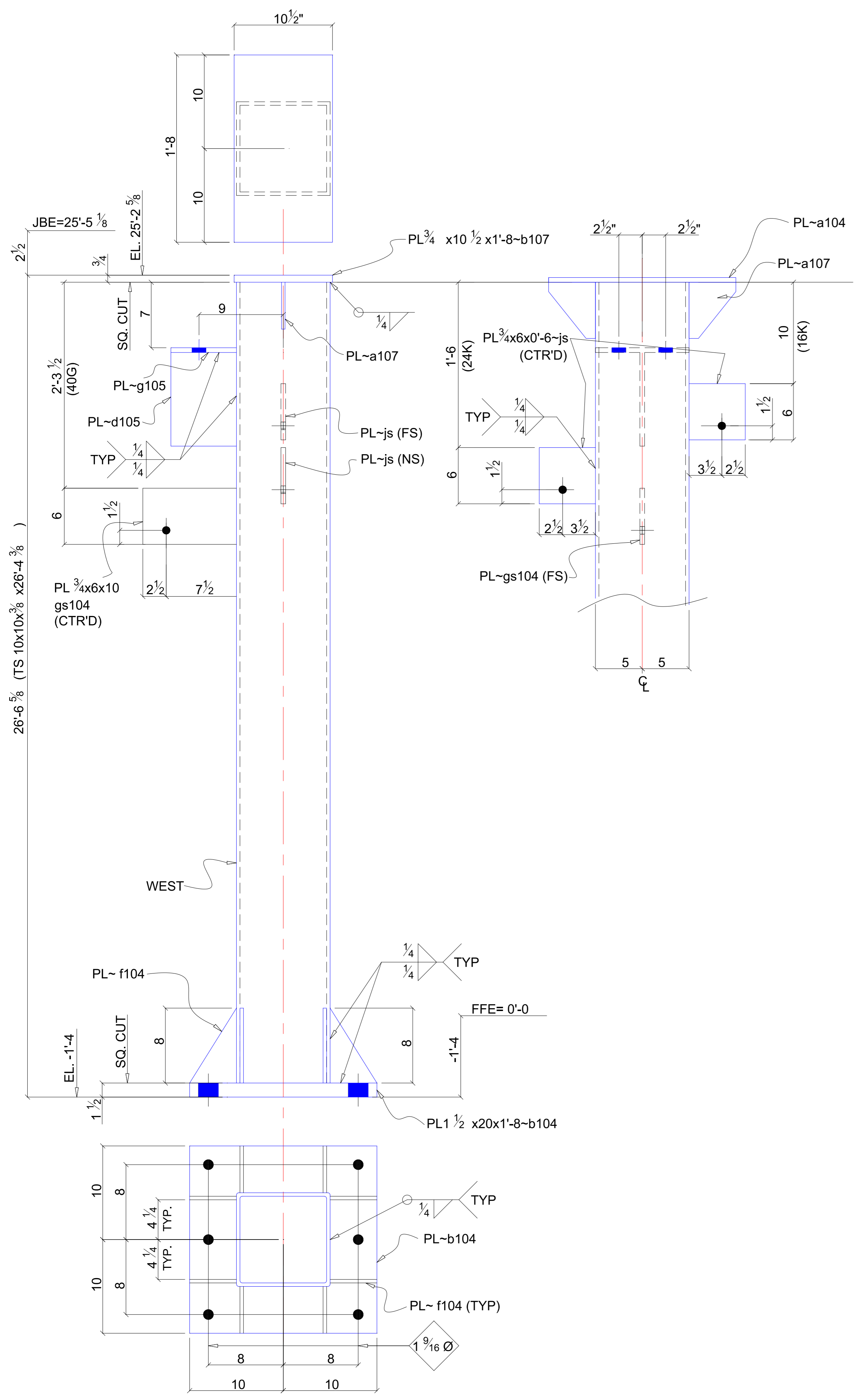
ONE-COLUMN MARKED ~A105 (@ GRIDS 5/N)
