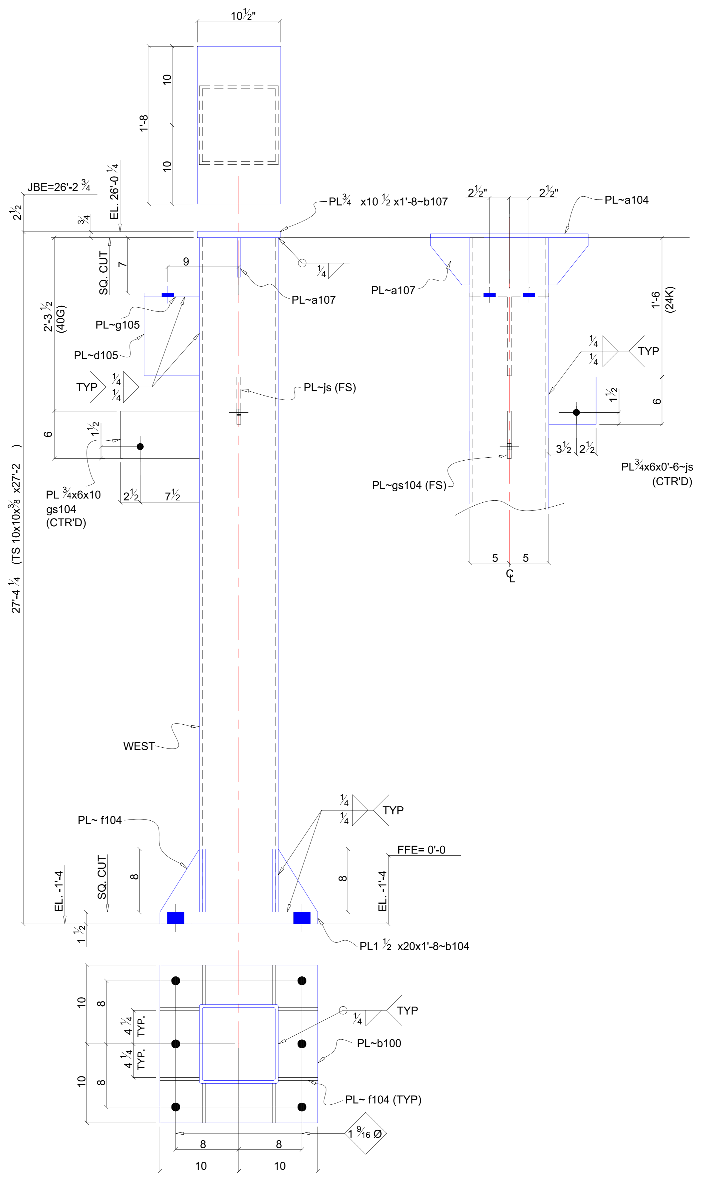
ONE-COLUMN MARKED ~B105 (@ GRIDS 4.03/N)
