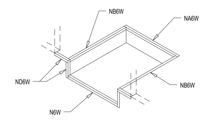
DETAIL OF DOCK LEVELER PIT
